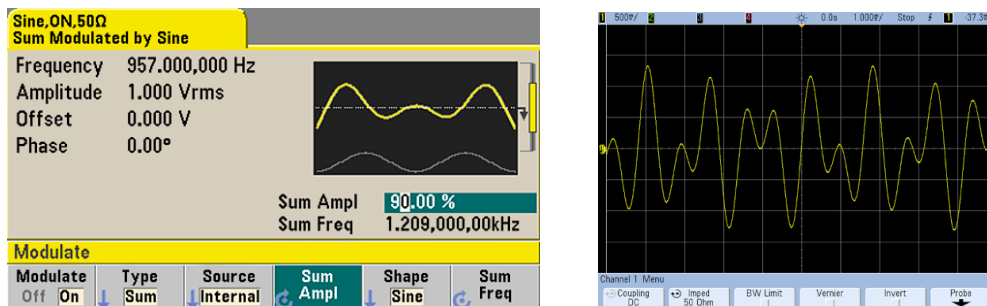
The dual-tone signal created by summing waveforms using the modulation type “Sum.”
