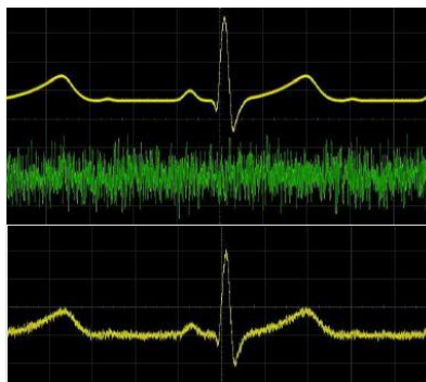
Add variable BW noise to any signal.
